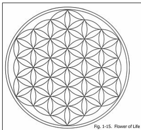
Fig. 1-15. Flower of Life
