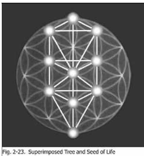
Fig. 2-23. Superimposed Tree and Seed of Life
